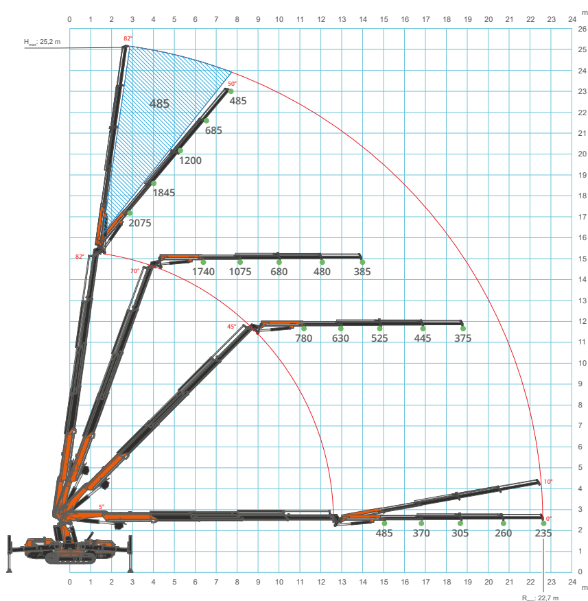
Hydraulic Jib
